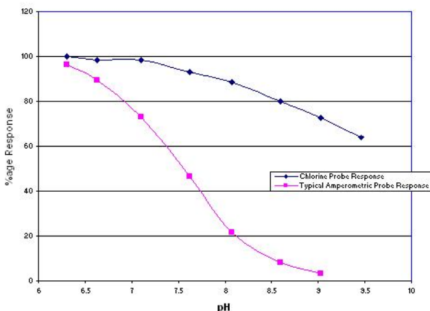
Typical Probe Response to pH (Unbuffered)
